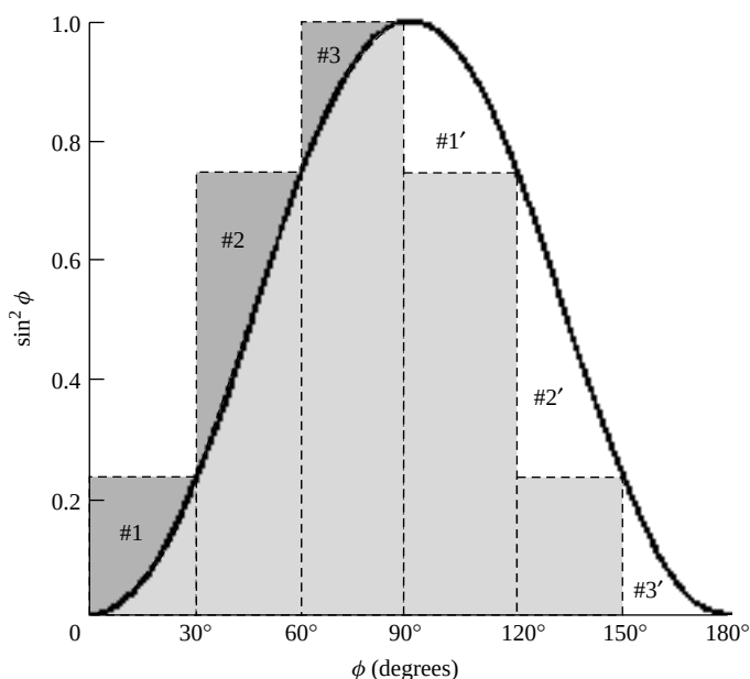
Figure 2.21 Digitized form of \sin^2 \phi function.
