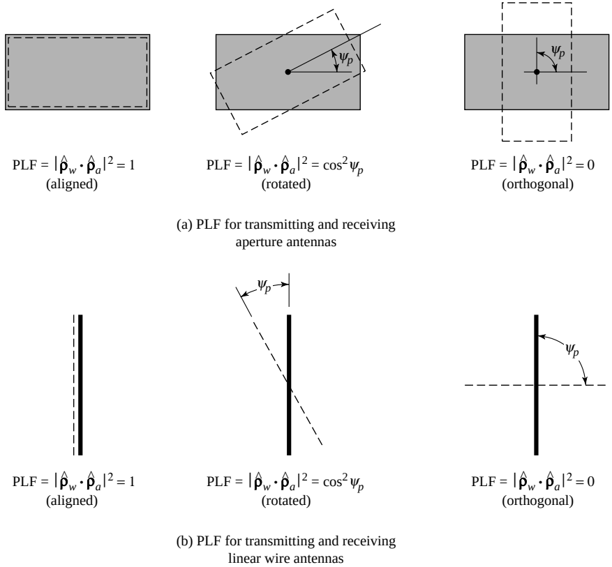
Figure 2.25 Polarization loss factors (PLF) for aperture and linear wire antennas.
