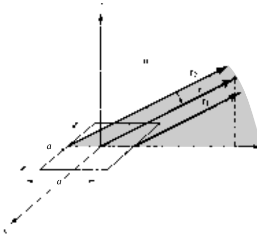
Figure 5.17 Square loop geometry for far-field observations on the y - z plane.
