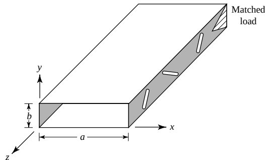
(b) Sidewall—inclined
