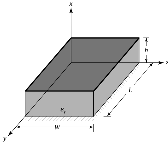
Figure 14.13 Rectangular microstrip patch geometry.
