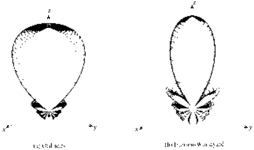
Figure 6.13 Three-dimensional patterns for ordinary and Hansen-Woodyard end-fire designs ( N = 10 , d = \lambda/4 ).
