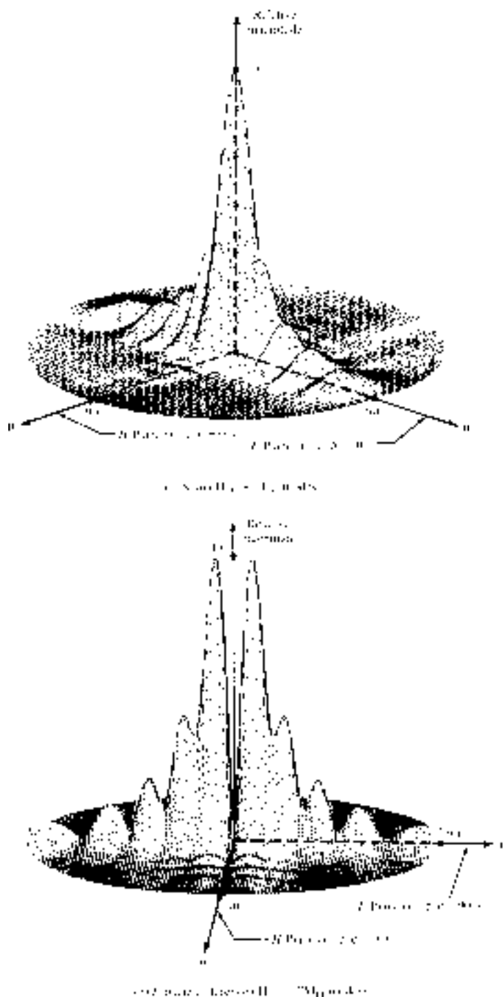
Figure 13.35 Three-dimensional sum and difference ( E - and H -planes) field patterns of a monopulse pyramidal horn. (SOURCE: C. A. Balanis, "Horn Antennas," in Antenna Handbook (Y. T. Lo and S. W. Lee, eds.), © 1988, Van Nostrand Reinhold Co., Inc.)
