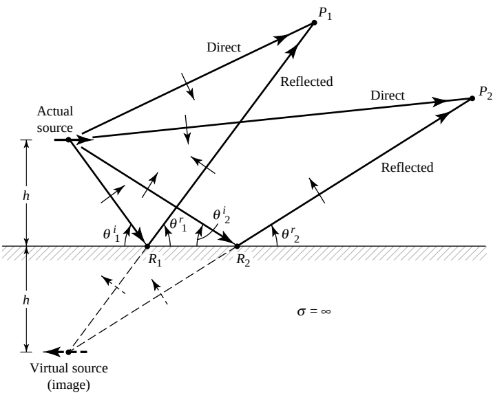
Figure 4.24 Horizontal electric dipole, and its associated image, above an infinite, flat, perfect electric conductor.
