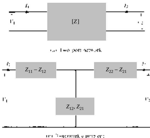
Figure 8.18 Two-port network and its T -equivalent.
