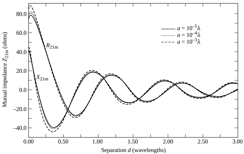
(a) Side-by-side
