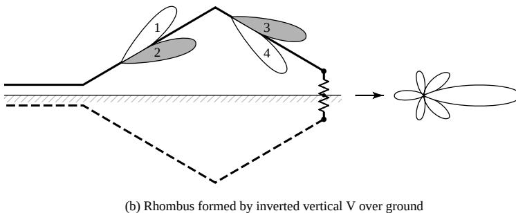
Figure 10.12 Rhombic antenna configurations.
