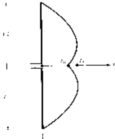
Figure 4.10 Current distribution of a linear wire antenna when current maximum does not occur at the input terminals.
